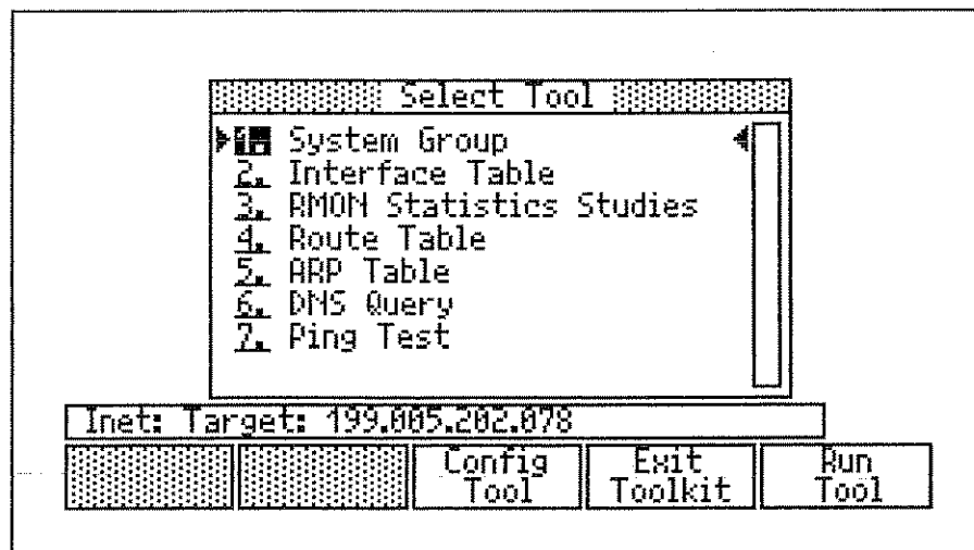
Figure 8-4. Toolkit Menu
